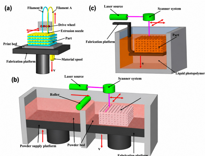
Figure 2. SLA uses a laser to polymerize liquid photopolymer resin SLA: Stereolithography
