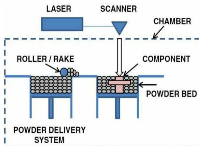
Figure 3. SLS procedure principle 5
